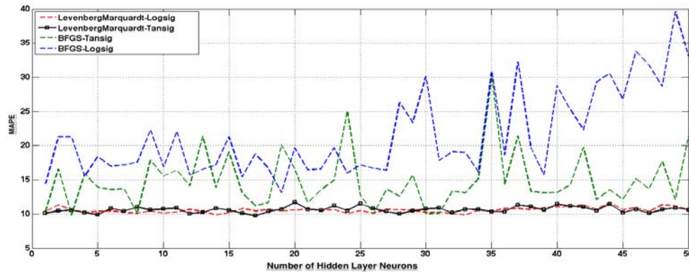
Fig. 9. Number of hidden layer neurons and transfer functions price forecast results
