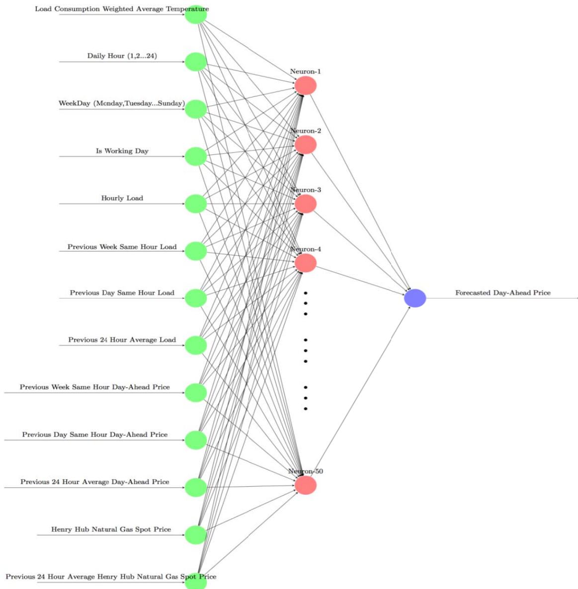
Fig. 6. Electricity price forecast neural networks models
