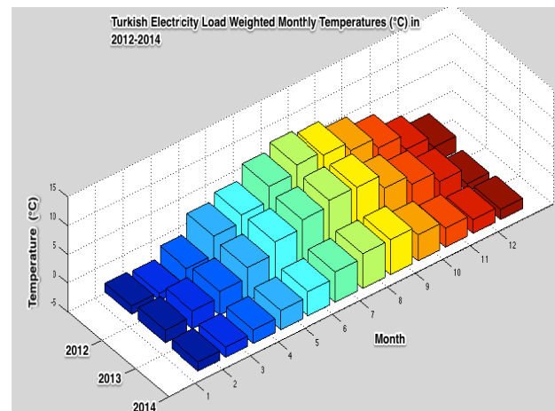
Fig. 5. Turkey electric load weighted monthly temperatures
