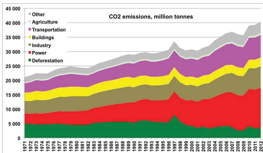
Fig. 1. CO 2 emissions by activity since 1971
