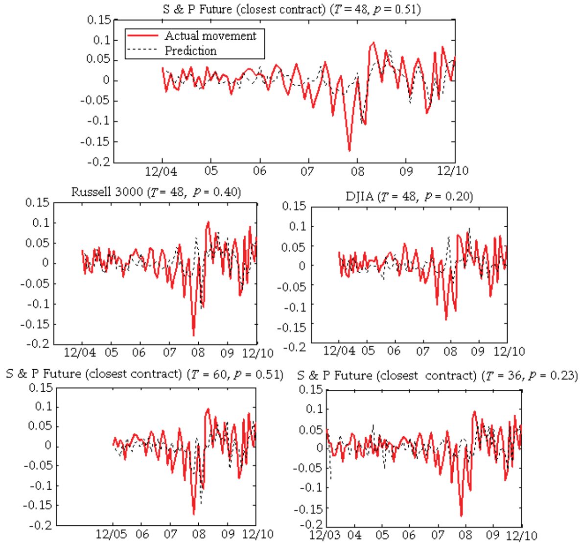
Fig. 5. Out-of-model prediction in rolling regression
