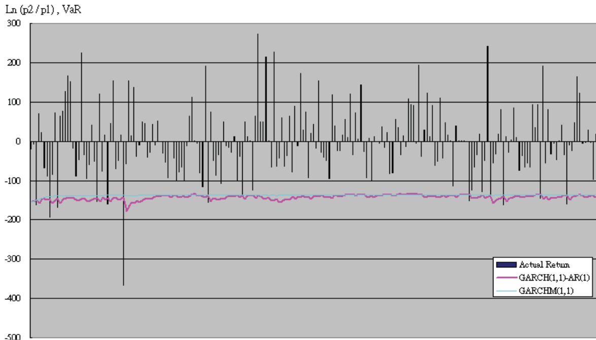
Fig. 5. The actual returns and the VaR of portfolio A
