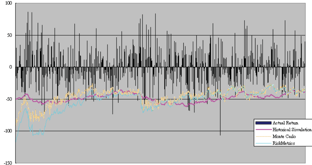
Fig. 3. The actual returns and the VaR of portfolio A
