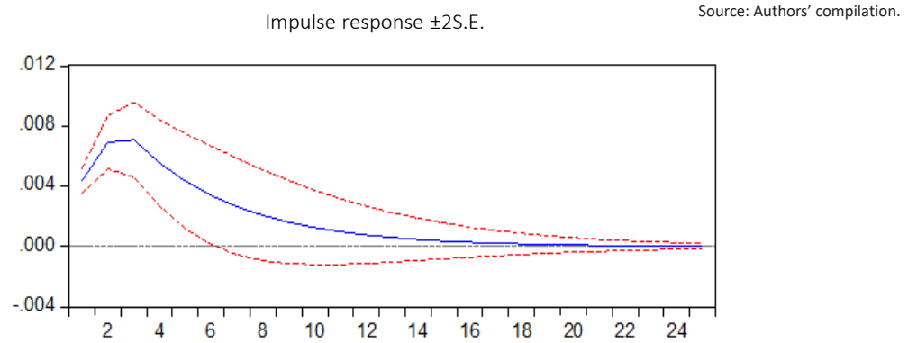
Figure 6. The impulse response of the model ARMA (1,2)
