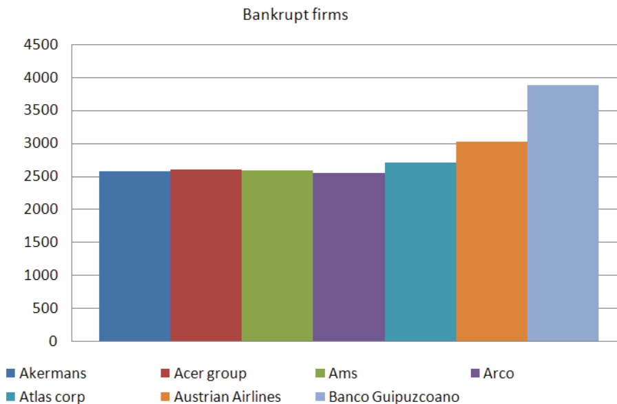
Fig. 3. EDF of bankrupt firms during the first year of forecast
