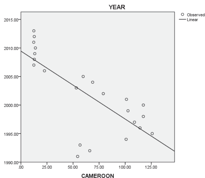
Fig.1. Regression equation
