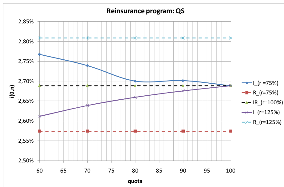
Fig. 2. Performance index i(0, n) for QS treaty
