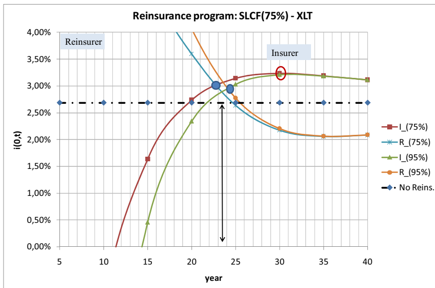
Fig. 8. Index i(0, t) . Hp.: Percentile SLCF \gamma = 75\% and \varphi(M; T) = 2,5\%
