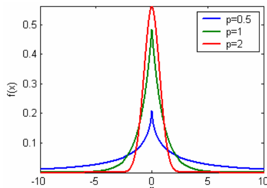
Fig. 1. Generalized Gaussian Distribution
