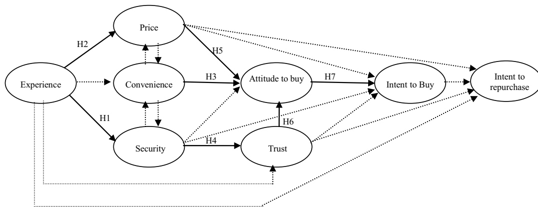
Fig. 2. Research Model
