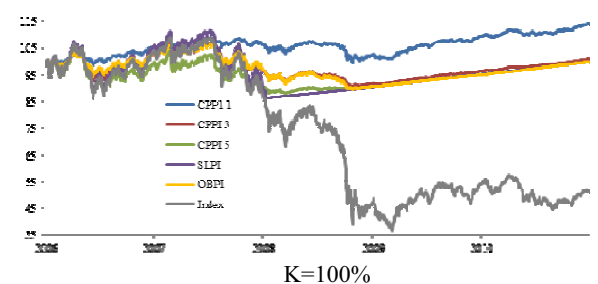
Fig. 3. Strategies performance in Nikkei 225
