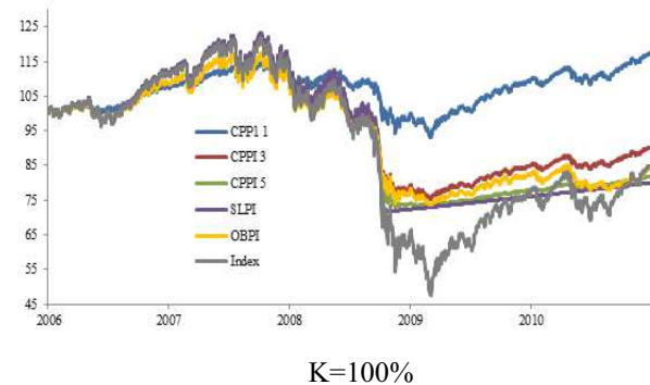
Fig. 1. Strategies performance in S&P 500
