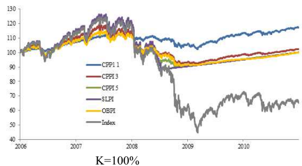
Fig. 2. Strategies performance in DJ EuroStoxx 50
