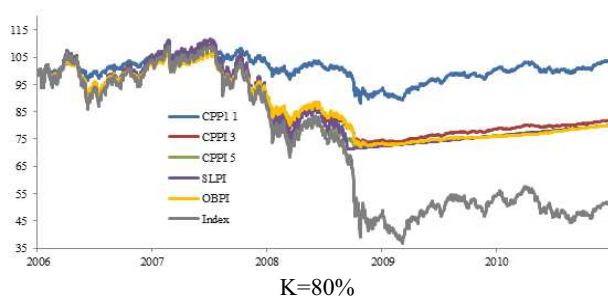
Fig. 3. Strategies performance in Nikkei 225
