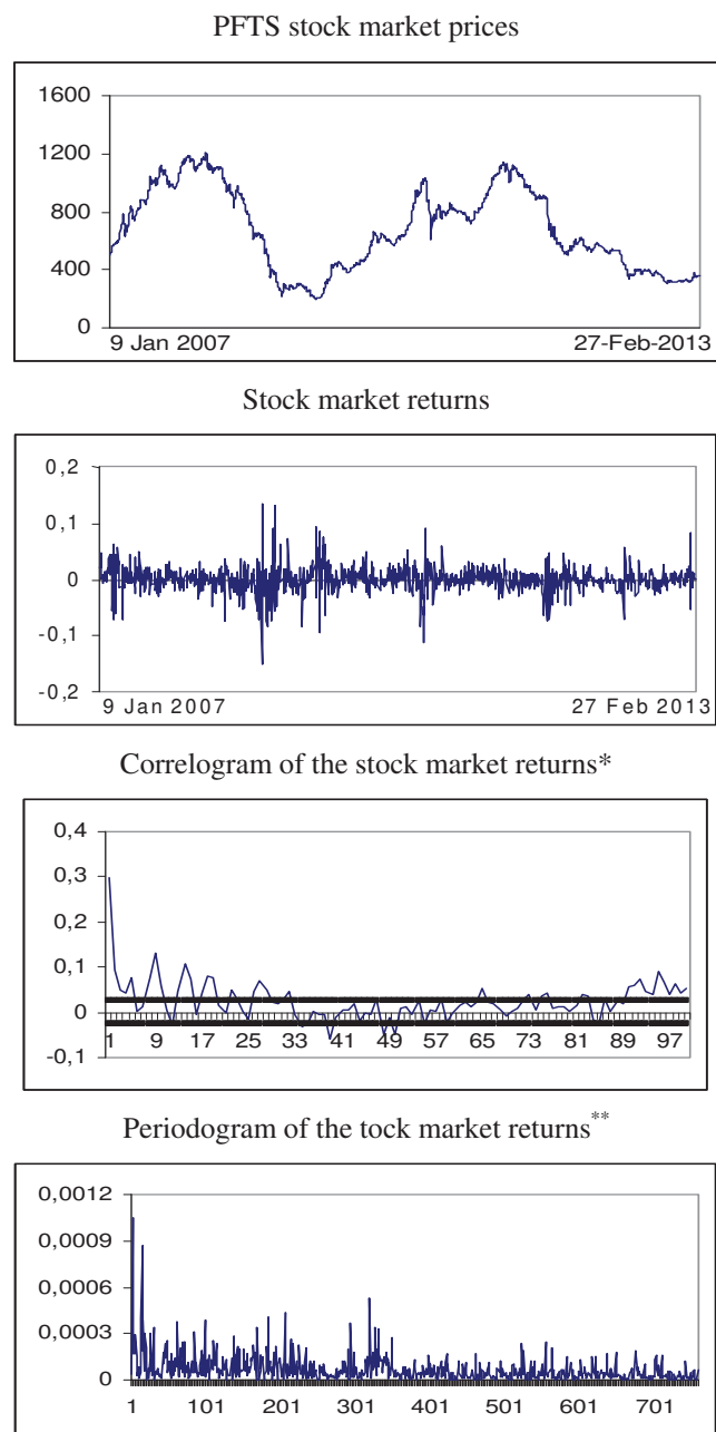
Fig. 1. Time series plots, correlograms and periodograms
