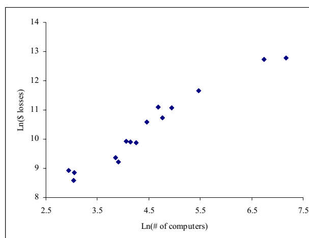
Fig. 1. Scatter plot $ losses versus # of computers on a logarithmic scale
