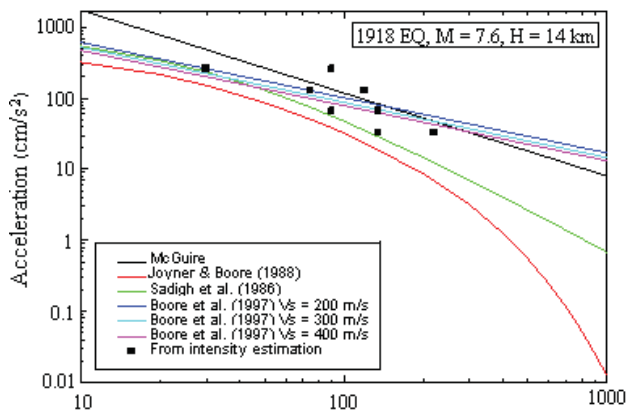
Fig. 14. Distance versus PGA values for 1918 Srimangal earthquake
