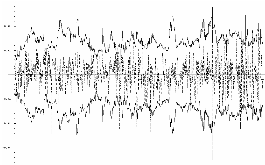
Fig. 1. VaR Bands of SEWMA model with varying \alpha . The lowest band represents the forecast 5% percentiles, whilst upper band represents the forecast 95% percentiles. The inner path shows sample data of the 4 th portfolio
