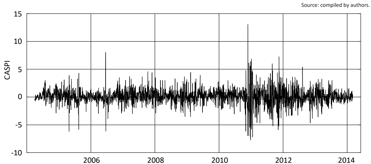
Figure 2. Frequent volatilities with extensive amplitude at DSE
