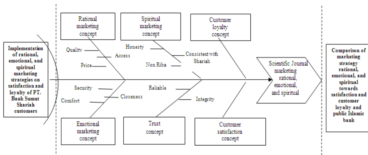
Fig. 2. Research flowchart
