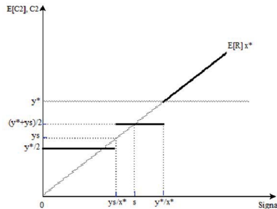
Fig. 3. Expected late consumption and observed signal with risk-neutral speculators (without central banker’s intervention)
