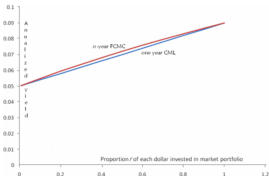
Fig. 2. The n -year FCMC for a 12-year risk-free ZCB, yielding 5 per cent per annum, and the market portfolio, yielding 9 per cent per annum
