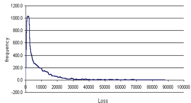
Fig. 1. Frequency distribution of Loss
