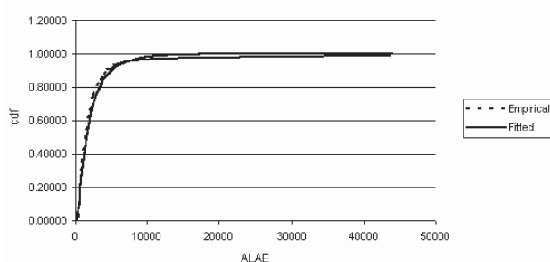
Fig. 5. Empirical distribution and fitted cdf of ALAE
