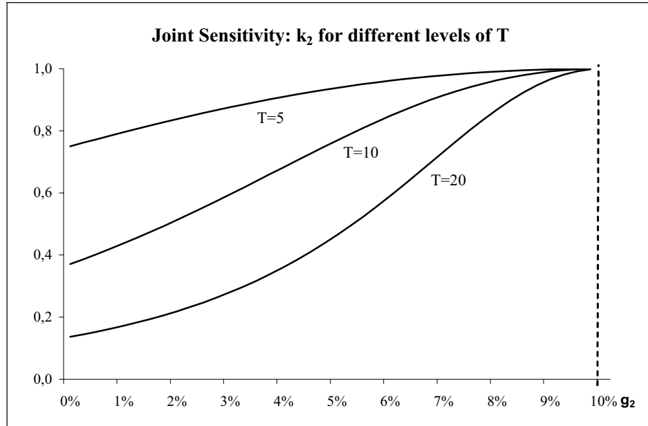
Fig. 4. Component of Joint Sensitivity due to g_2 , as a function of the length of the first stage
