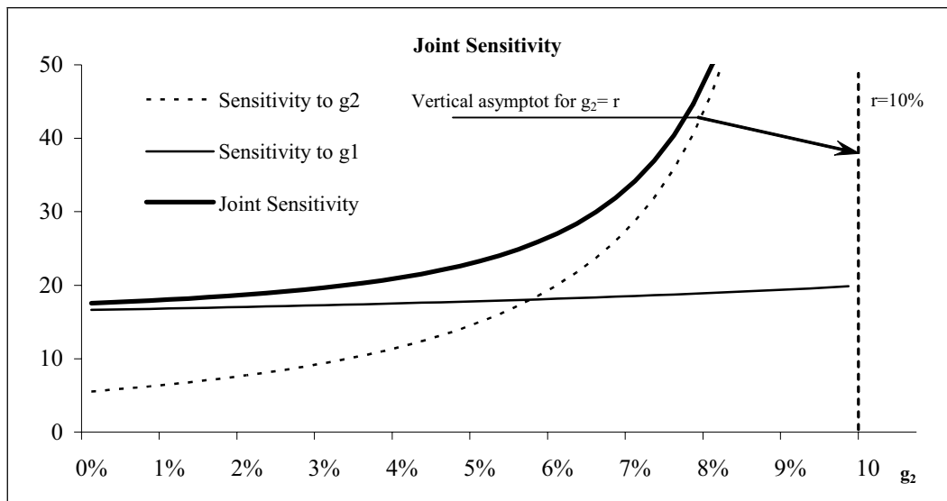
Fig. 3. Sensitivity to g_1 and g_2 and joint sensitivity for the two-stage model 1
