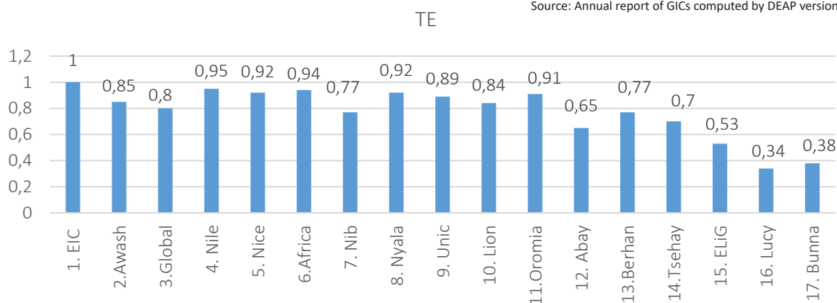
Figure 1. Relative technical efficiency score under CCR model
