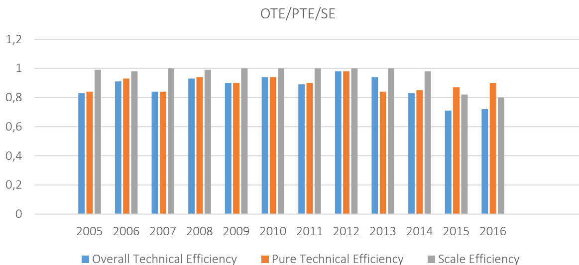
Figure 3. Average TE, PTE, and SE
