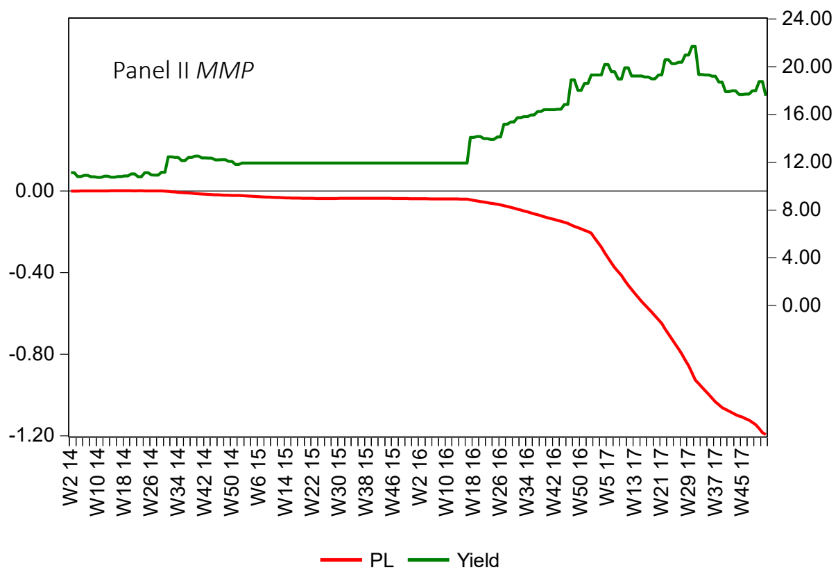
Figure 3. Floating yields Y_{i,t}^F (%) and profits/losses PL_{i,t} (EGP) for selected simulated portfolios MMP_i
