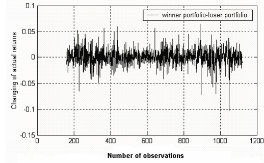
Fig. 4. Momentum profits for the R-Ratio (0.3, 0.4) on a 6-month ranking period
