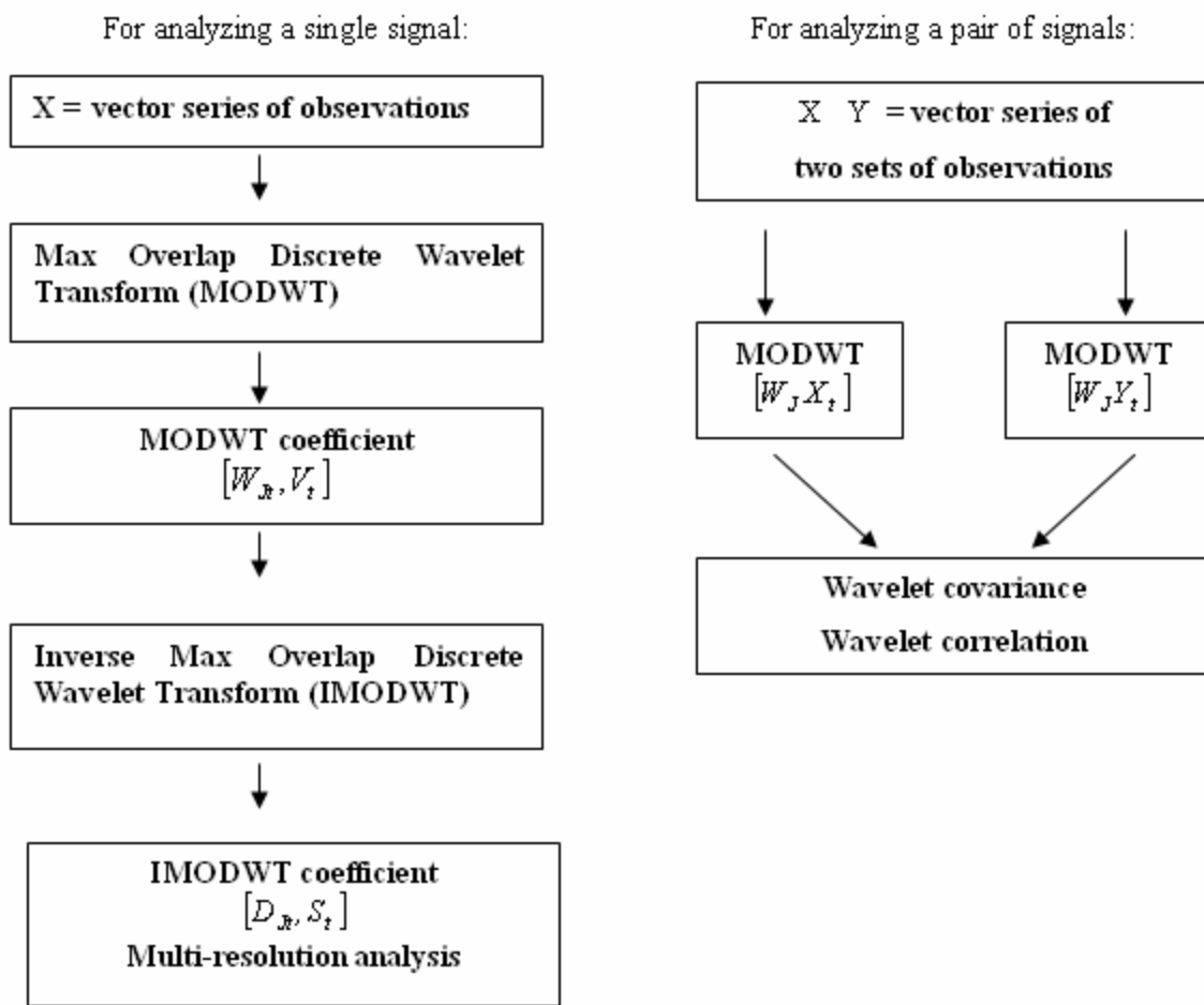
Fig. 1. MODWT Workflow
