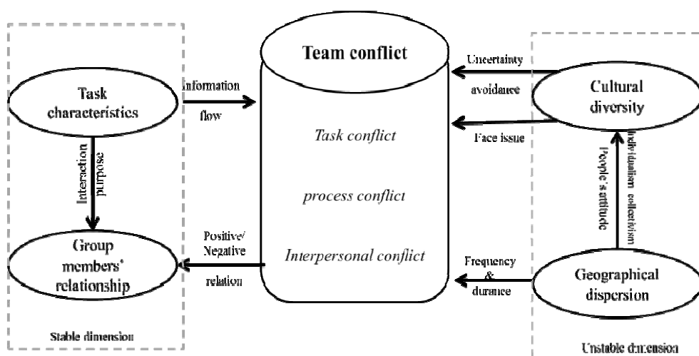
Figure 11 Conceptual framework
